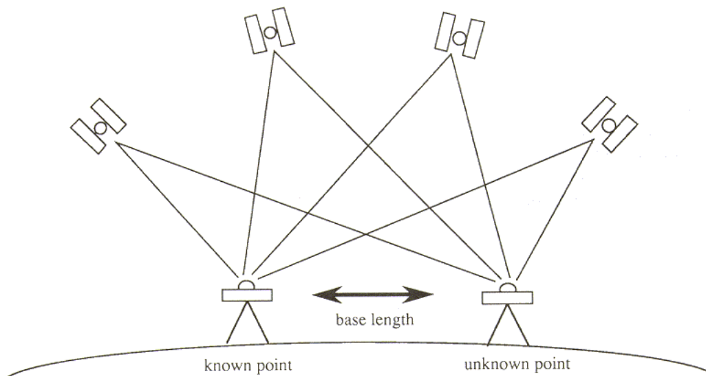
Figure 6.8.2 Relative positioning
