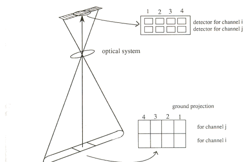
Figure 6.2.2 Relationship between a detector and its ground projection
