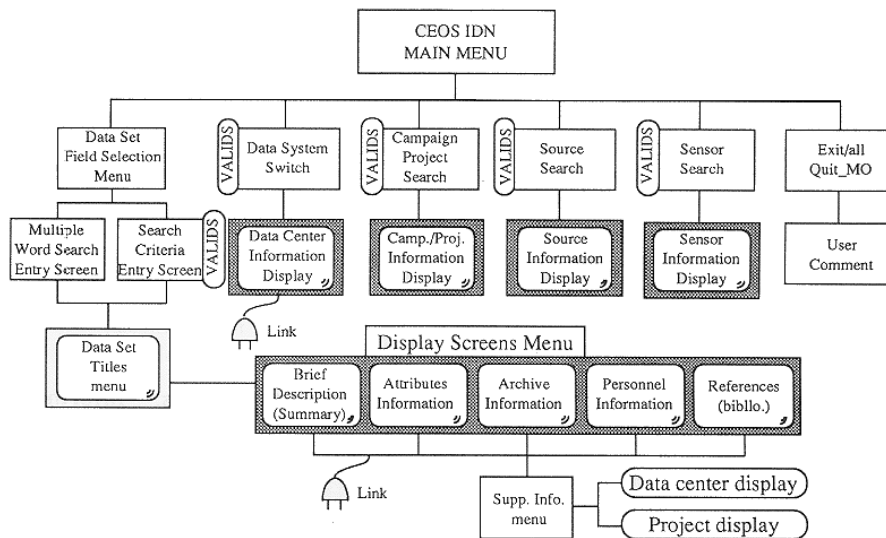
Fig. 6.13.1 Main Menu of CEOS IDN
