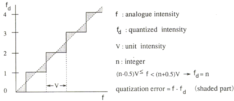
Figure 6.1.2 Concept of quantization
