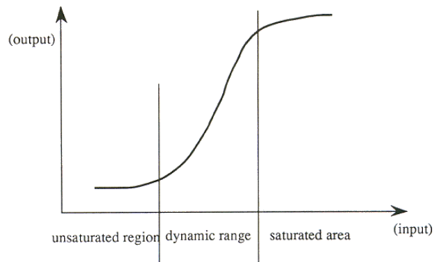
Figure 6.3.1 Input-output characteristic curve
