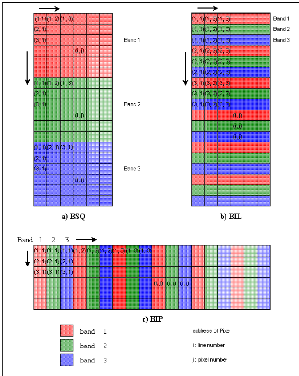
Figure 6.4.1 Image data format (in the case of 3 separate bands)
