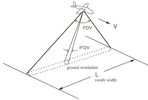
Figure 6.2.1 FOV and IFOV
